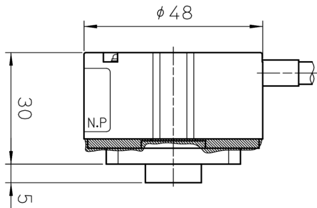
(c) 编码器侧视图
