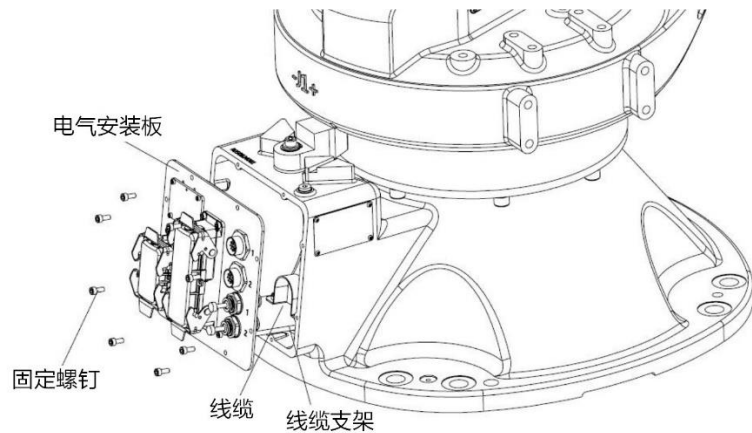
图 12-4 AIR50-2260/AIR80-2260/AIR35-2700/AIR20-3100 底座内部线缆
