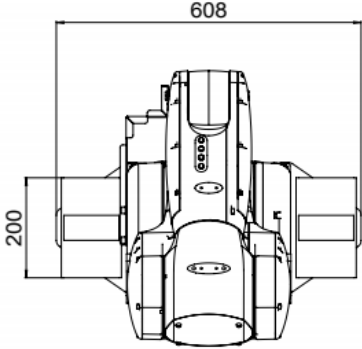
(c) 俯视图
