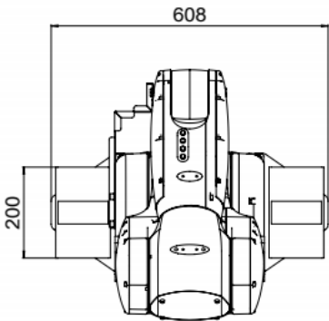
(c) 俯视图
