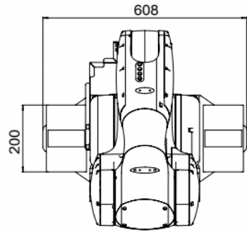
(c) 俯视图
